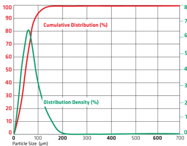
2924 Particle Size Distribution
