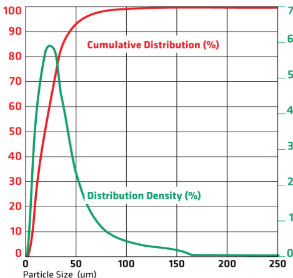
5935 Particle Size Distribution
